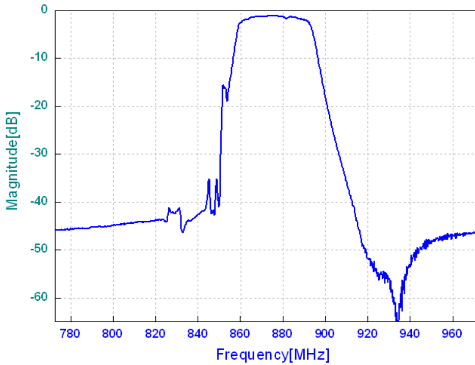
Frequency Response
